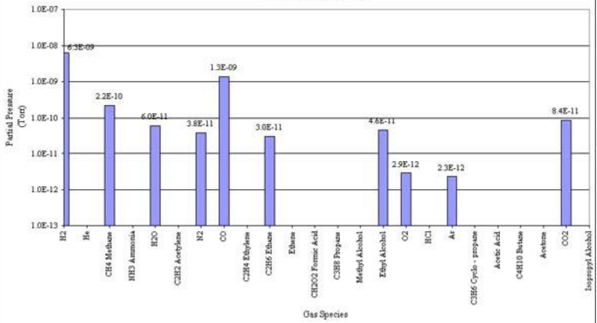
Partial Pressures of Constituent Gases for Flex Strip Sample 2 Test
